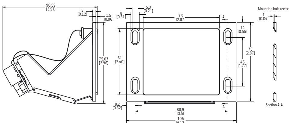
Figure 1. Mounting and Dimensional Drawing (For reference only: mm/[in])
